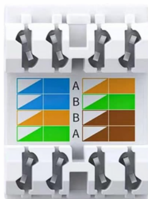
Standard 568B
